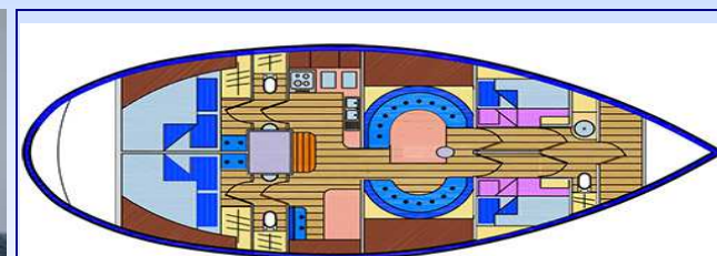
Beneteau First 45.6
